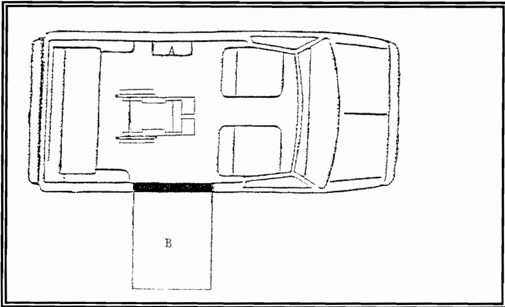
A. 1-2 Passenger Flip Seat, B. Ramp
